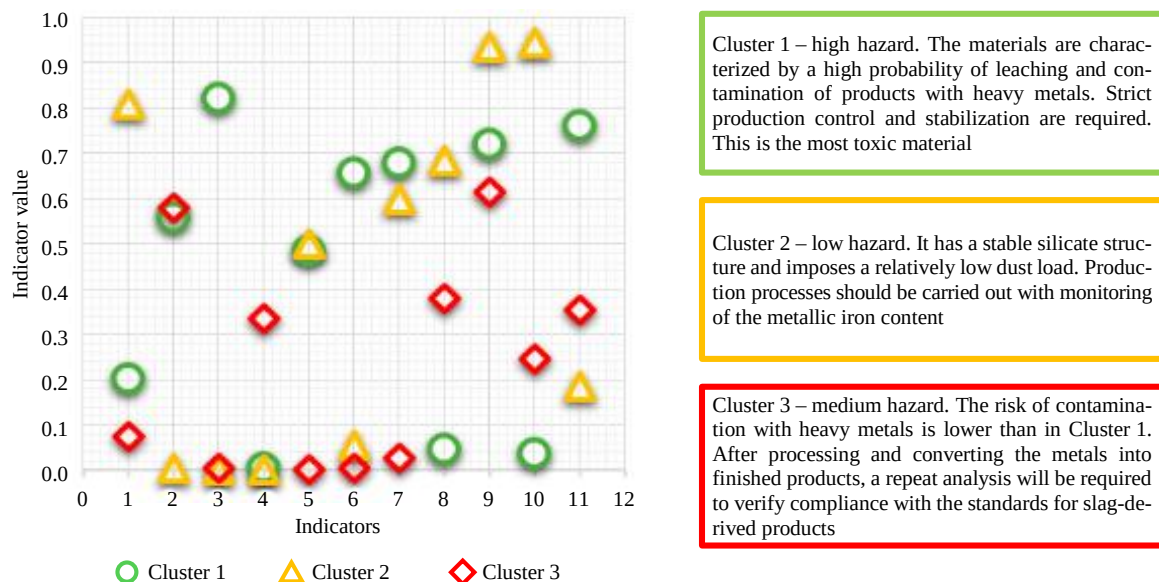
Fig.4. Mean values of environmental indicators for various clusters: 1 – Fe_{met} ; 2 – S ; 3 – Pb ; 4 – Cr ; 5 – Zn ; 6 – Cu ; 7 – Ni ; 8 – MnO ; 9 – crystallinity; 10 – basicity modulus; 11 – content of 0-5 mm fraction grains, %
