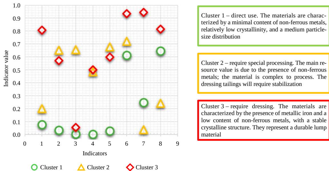
Fig.3. Mean values of resource indicators for various clusters: 1 – Fe_{met} ; 2 – FeO ; 3 – Cu ; 4 – Zn ; 5 – Ni ; 6 – crystallinity, %; 7 – basicity modulus; 8 – content of 5-70 mm fraction grains, %
