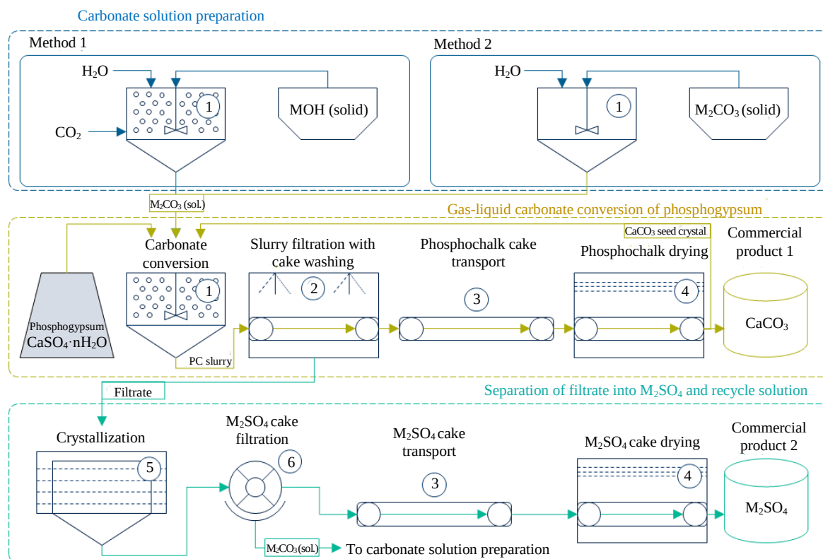
1 – mixing reactor; 2 – belt vacuum filter with precipitate washing; 3 – belt conveyor; 4 – belt dryer; 5 – crystallization reactor with cooling; 6 – vacuum filter
