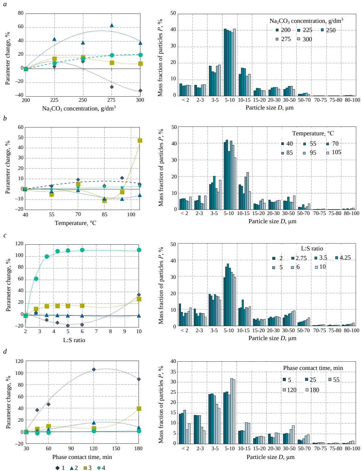
Fig.3. Variation of the main process parameters as a function of the variable factors: a – effect of \text{Na}_2\text{CO}_3 concentration; b – effect of conversion temperature; c – effect of liquid-to-solid ratio; d – effect of phase contact time 1 – filtration rate; 2 – particle size D50; 3 – particle size D90; 4 – conversion degree
