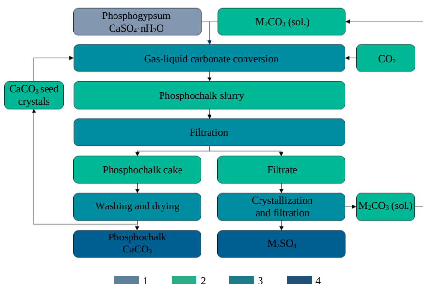
Fig.2. Schematic diagram of the PG carbonate conversion process
