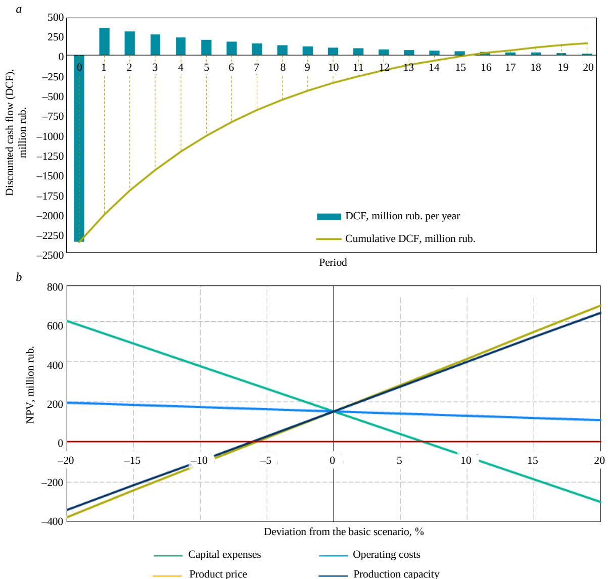
Fig.5. Results of economic efficiency assessment (a) and sensitivity analysis (b)
