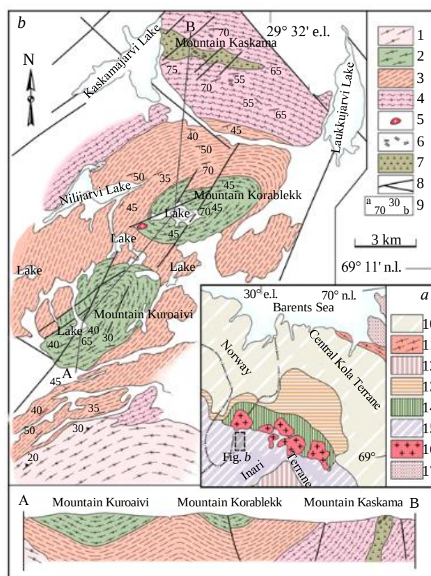
Fig.1. A geological scheme of the Kaskama structure [35] with corrections
