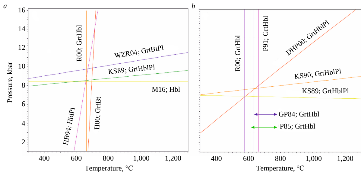
Fig.6. PT-diagrams with the results of calculation of metamorphism parameters of the studied schists: a – samp. 17-4a (migmatized garnet-amphibole-plagioclase schist); b – samp. 8-6 (amphibole-plagioclase schist). Calculation lines for mineral thermometers and barometers correspond to: GP84 [18], P85 [19], KS89 [24], KS90 [25], P91 [20], HB94 [17], H00 [22], DHP00 [26], R00 [21], WZR04 [27], M16 [23]
