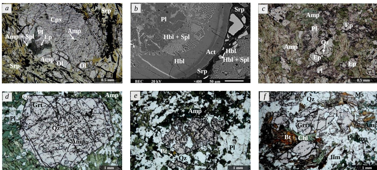
Fig.2. Microphotographs of thin sections in transmitted light (a, c-f) and BSE (b) of the Kaskama Formation rocks: a – metamorphosed peridotite (samp. 104), serpentinized Ol, Cpx replacing Hbl, Ep replacing Pl, Spl+Hbl symplectites after Pl; b – metamorphosed peridotite (samp. 104), Spl+Hbl symplectites, zonal Amp border at the contact of Ol with Pl; c – epidote-bearing amphibolite (samp. 8-12), epidote grains contain quartz inclusions, plagioclase is altered; d – garnet-amphibole schist (samp. 101-1), Grt with formed facets contains Qz and Amp inclusions, enveloped by prismatic light-green Amp; e, f – migmatized garnet-amphibole-plagioclase schist (samp. 17-4a), Grt in Pl-Amp matrix, replaced by Chl-Bt-Ms aggregate, contains Qz and Pl inclusions
